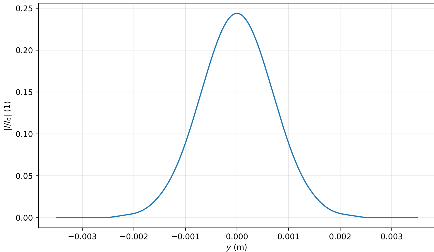
Intensity profile I(x=0, y, z=3.742)/I_0 , P_{in}=0.1P_{cr} , artificial time
